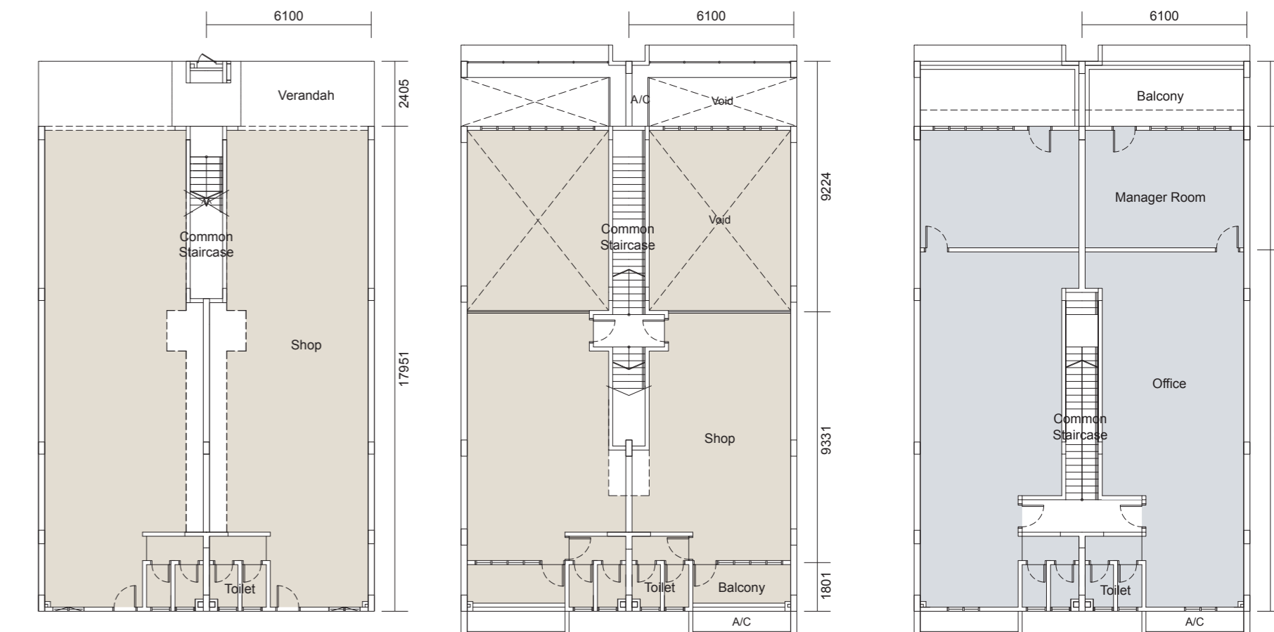
Ground & Mezzanine Floor Built-up Area: 1,830 - 2,745 sq.ft.
